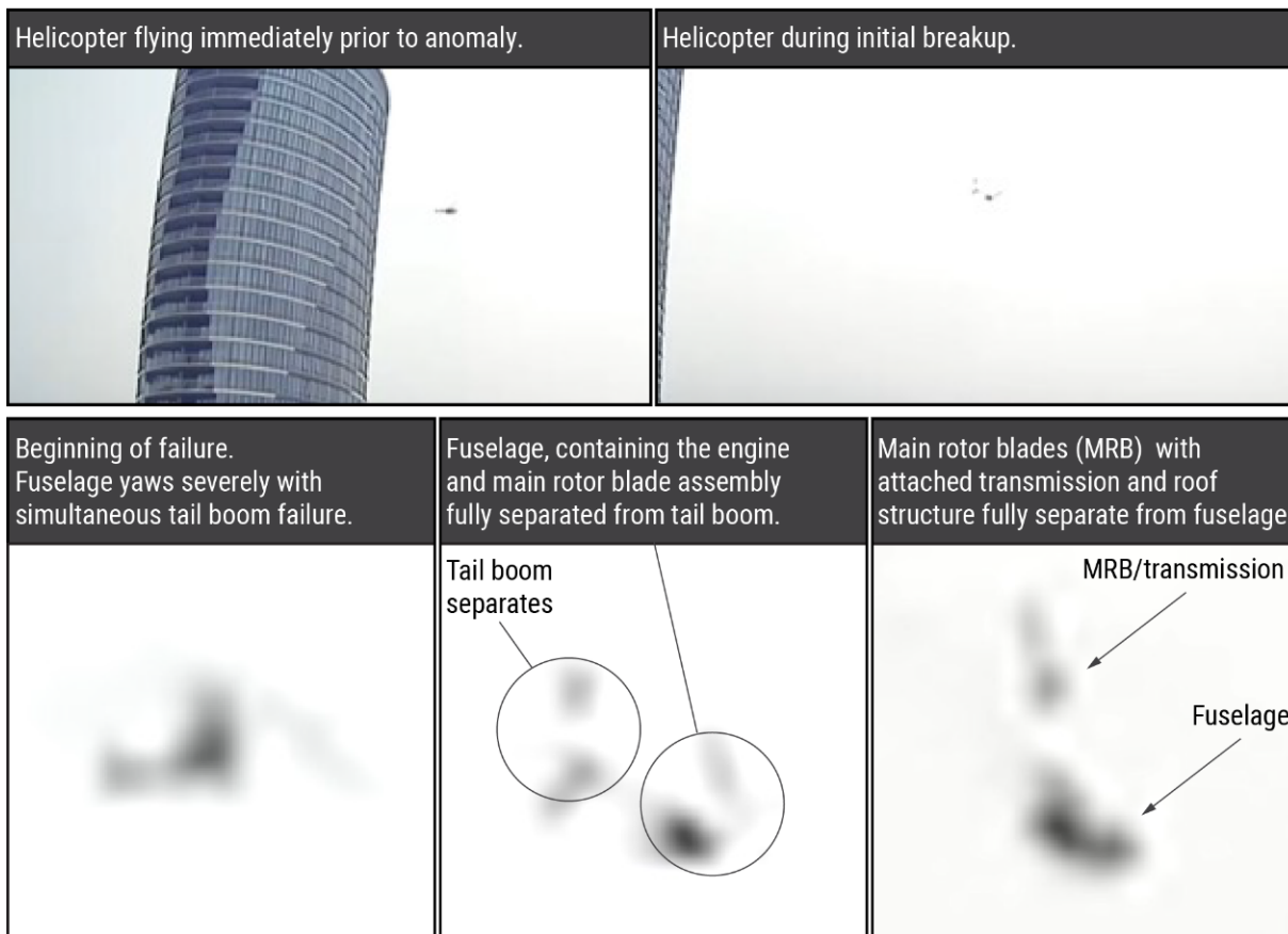
Figure 3. Enhanced surveillance video with sequential images depicting the helicopter's flight and breakup.
